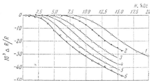
FIG. 4. Dependence of \Delta R/R on H . Curve 1 — atmospheric pressure; curves 2–6 at pressures ( P ) 2600 , 5400 , 7025 , 8850 , and 10800 \text{ kg/cm}^2 , respectively.
